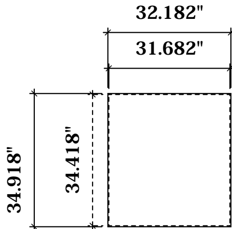
Pedestal Front Infill 1/8" Substrate
